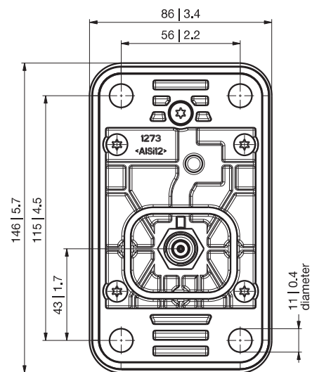
Mounting flange:
