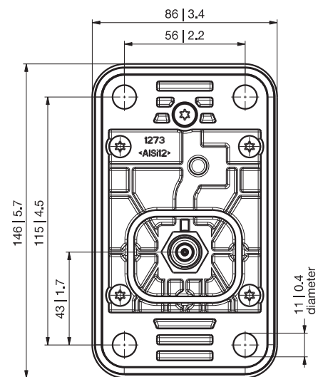
Mounting flange:
