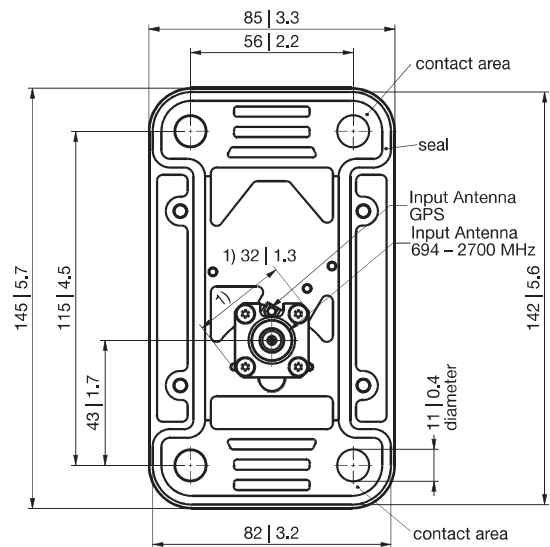
Mounting flange:
